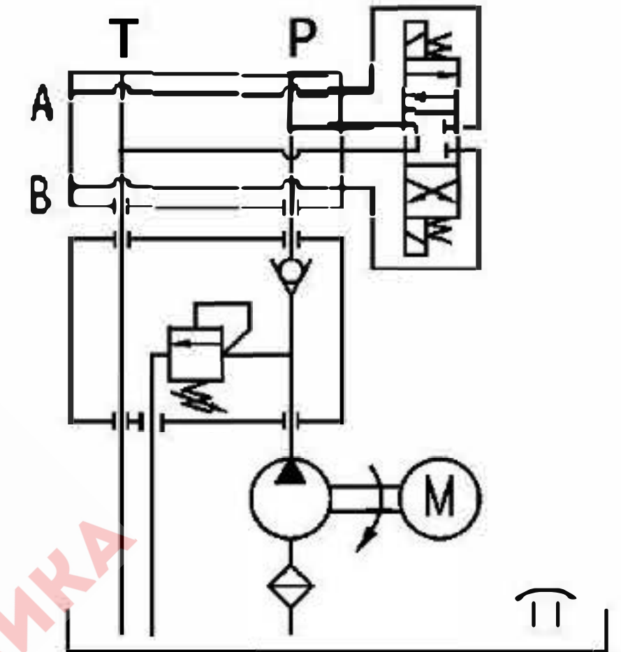
HYDRAULIC CIRCUIT
