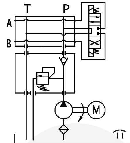
HYDRAULIC CIRCUIT
